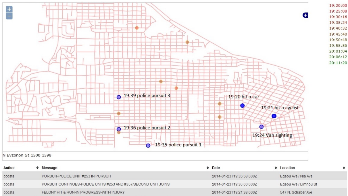
Figure 3: Geo-spatial view. Messages are shown as dots and colored according to time (legend in the top-right corner). The details of the selected messages are shown as a list at the bottom.
